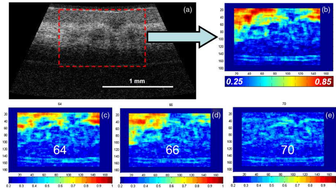
Fig. 12 An in vivo example of elastographic CS mapping performed at the speckle level for a human finger-pad skin. (a) Initial OCT image exhibiting peculiar speckle structure and corresponding to B-scan number 65 that is chosen as a reference one. The boundary between the upper corneous layer of the skin (stratum corneum) and deeper located softer epidermis (that looks lighter in the intensity image) is visible due to somewhat different scattering properties of the subresolution scatterers. (b) The resulting elastographic CS image obtained by averaging the CS maps for the B-scans number 64 and 66 (i.e., just before and just after the reference frame number 65). Panels (c) through (e) are the examples of individual CS maps obtained via cross-correlating the reference image number 65 with the neighboring B-scans number 64, 66, and 70. The upper stiffer layer in the CS maps for B-scans number 64 and 66 is quite clearly seen due to significantly higher cross-correlation coefficient. For the stronger deformed frame number 70, the speckle-level cross-correlation is strongly reduced practically down to the background level even within the stiffer upper layer. The acquisition rate for the discussed sequence is 10 f/s. The images were recorded in free-hand mode.
