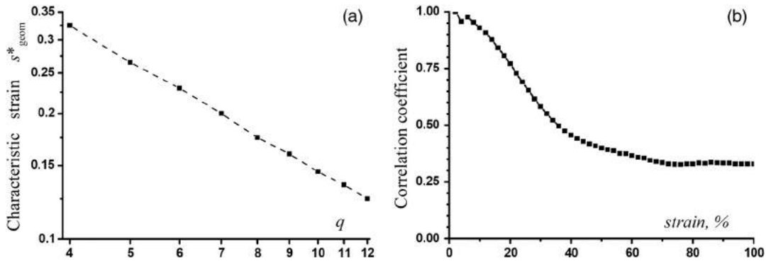
Fig. 2 Simulation results for the cross-correlation decrease due to purely geometrical distortion of the image. (a) The characteristic strain s_{geom}^* as a function of quantity q found for a rectangular window containing q \times q independent elements and the assumed reduction in the cross-correlation by a factor of 2^{1/2} under compressional deformation produced by uniaxial stress. (b) Correlation coefficient (1) for a reference and deformed images as a function of strain found for shear-type deformation and the parameter q = 4 .
